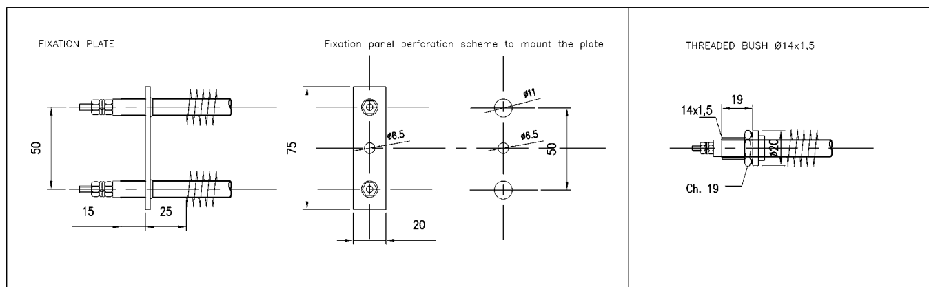
Figure 5: dimensions and constructive characteristics of fixation devices for elements with sheath diameter 10 mm
